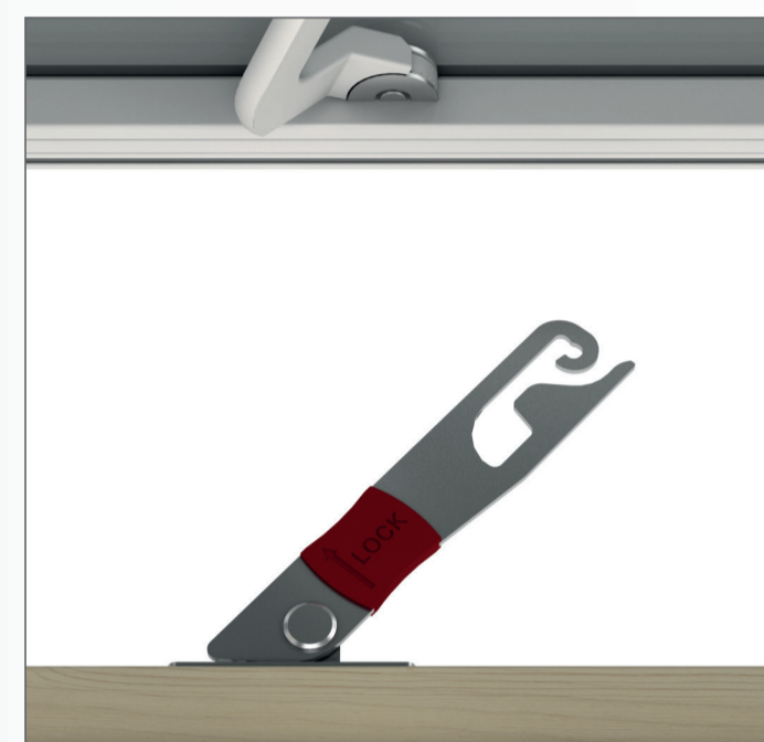
Standard restrictor w/ventilation position lock. Not available for sliding casement door.
